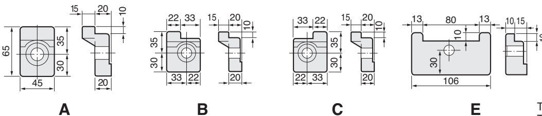
T-slot pitch guide piece
