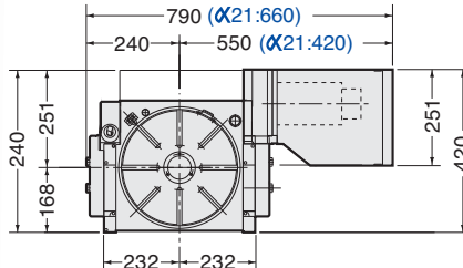
Guide key width: 18mm Table height in horizontal position: 182mm
