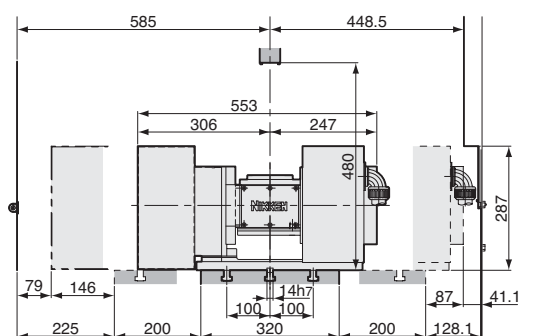
5AX-130SA-BR on TC-S2D
