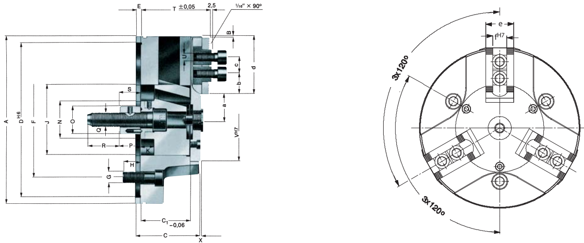
3-jaw power chuck, weight reduced, serration 90° Adaptor recess, mounting dimensions to DIN 6353
